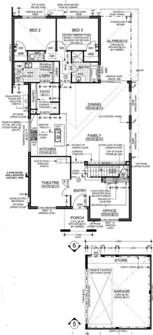
GROUND FLOOR
