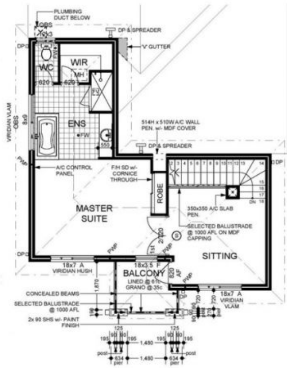
UPPER FLOOR
